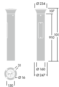
Borne Thor Slim
